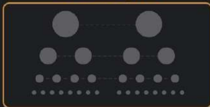
xGold Program
