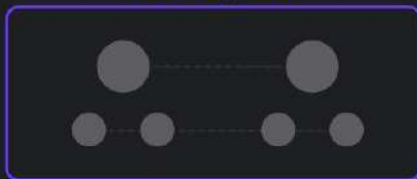
xGold Program
